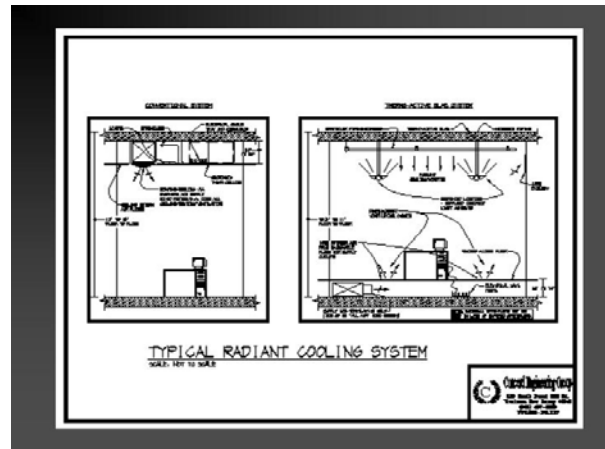
FIGURE 13 – TYPICAL RADIANT COOLING SYSTEM
