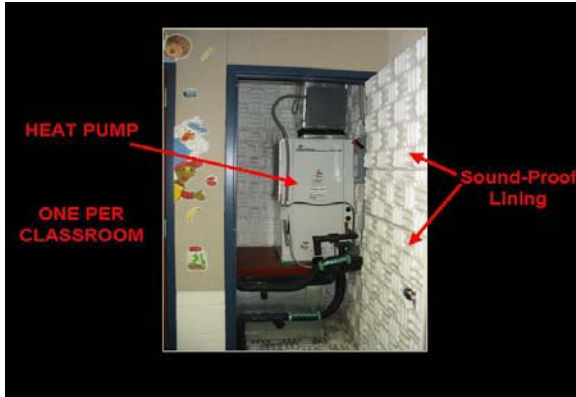
FIGURE 11 – HEAT PUMP
