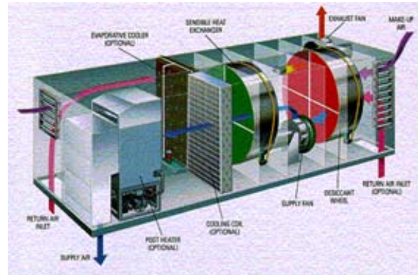
FIGURE 12 -DESSICANT ENERGY RECOVERY UNIT
