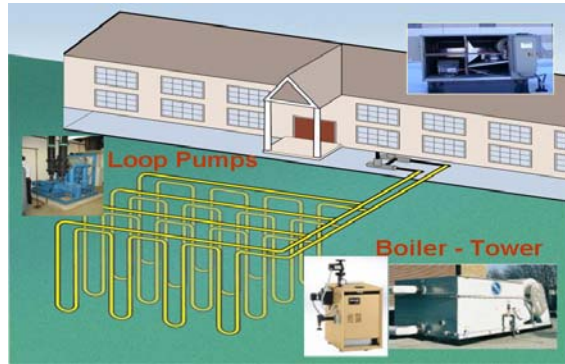
FIGURE 9 – WSHP & GSHP
