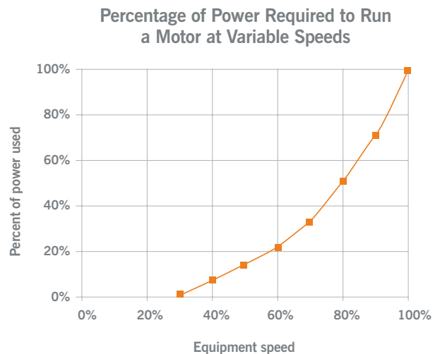
Figure 1: Percentage of power required to run a motor at variable speeds. Running equipment below full load saves energy because power consumption drops proportional to the cube of the motor speed. As an example of this, reducing the speed of an electric motor by one-third reduces its power consumption by 70 percent.
