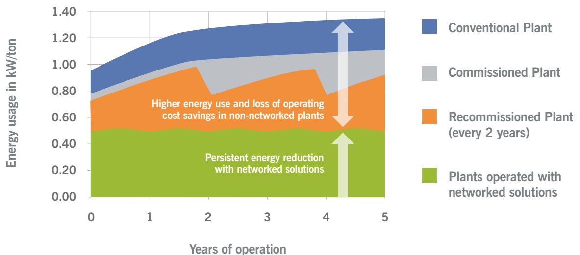
Figure 3: Commercial HVAC System Operating Efficiency. This chart compares plant performance using conventional control and maintenance processes versus plants that have been commissioned or recommissioned, and plants that use networked software solutions. Conventional plants and commissioned plants are subject to performance drift. Plants operated with networked software solutions have the real-time measurement, verification and management data needed to quickly detect, diagnose and repair system faults to ensure persistent energy reductions and operating cost savings.
