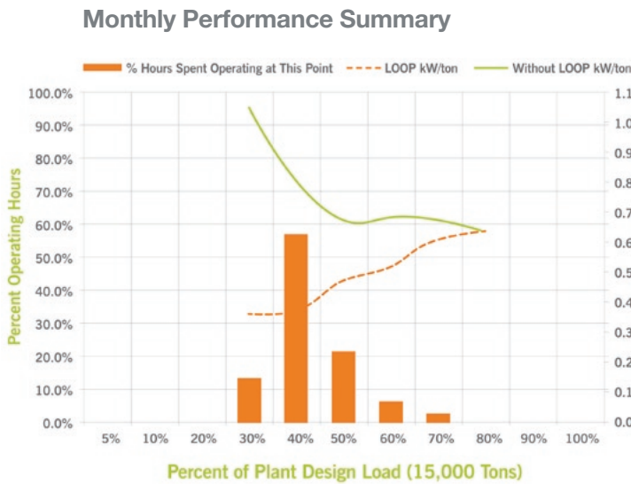
Figure 9: Monthly plant efficiency reports include graphical representation of key operating statistics. This Performance Summary shows that for about 70% of the total run hours, this plant was running between 30% to 40% of design load where the performance ranged from 0.32 to 0.35 kW/ton.
