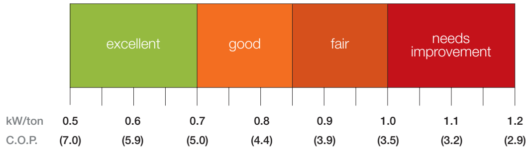
Figure 4: Ultra High Performance HVAC. Research has shown that plants operating for more than a few years typically have an annual wire-to-water operating range of 0.9 to 1.2 kW/ton. Variable speed plants that have undergone commissioning run more efficiently, often in the 0.7 to 0.8 kW/ton range. Ultra High Performance HVAC plants often achieve an average 0.5 kW/ton or less.
