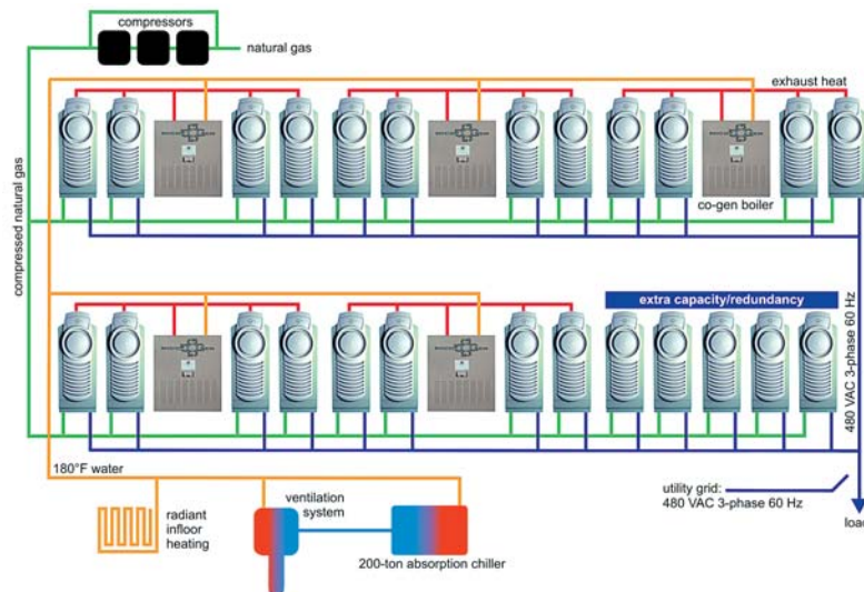
Anatomy of a Solution: A diagram of the system at Harbec Plastics.
